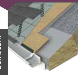
Box beam
